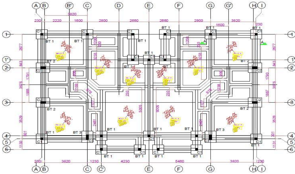
FOUNDATION LAYOUT
